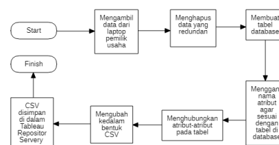
Gambar 7 Flowchart ETL
